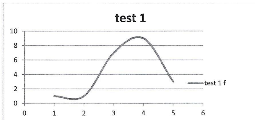
Figure No. 1. Skewness of Test One
