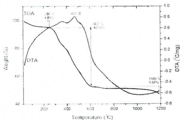
Fig. 1: TG-DTA plot of as-prepared sample Y_{3-x}Bi_xAl_{0.5}Fe_{4.5}O_{12} ( x = 1.0 ) composition
