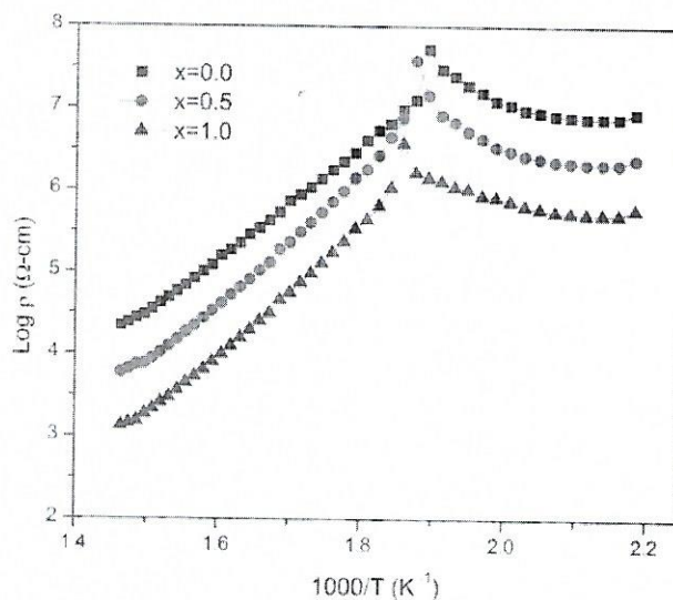
Fig. 3: Variation of \log \rho versus 1000/T for Y_{3-x}Bi_xAl_{0.5}Fe_{4.5}O_{12}
